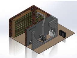
Floor mount
