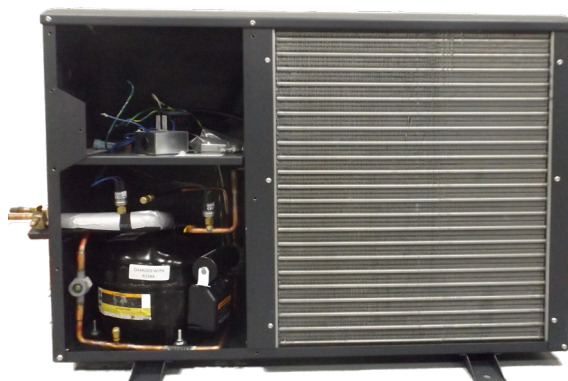
Condensing unit with easy-access cover
